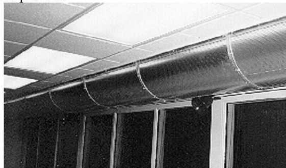
Figure 5 - Radial supply air plenum
